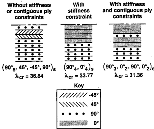
Fig. 4 Effect of stiffness requirement on laminate design for N_y/N_x = 2 and N_y = 2.0 lb/in. (350 N/m).
